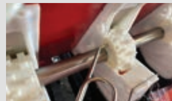
Dual large and fine metering wheels allow for a wide range of seed types and fertilisers
